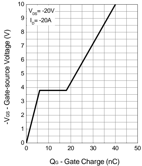
Gate Charge
